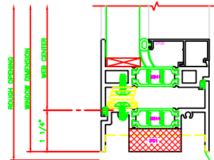
240 SILL 325 CASEMENT OUT 4-BAR ARMS
