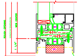
241 SILL 325 CASEMENT OUT BUTT HINGES
